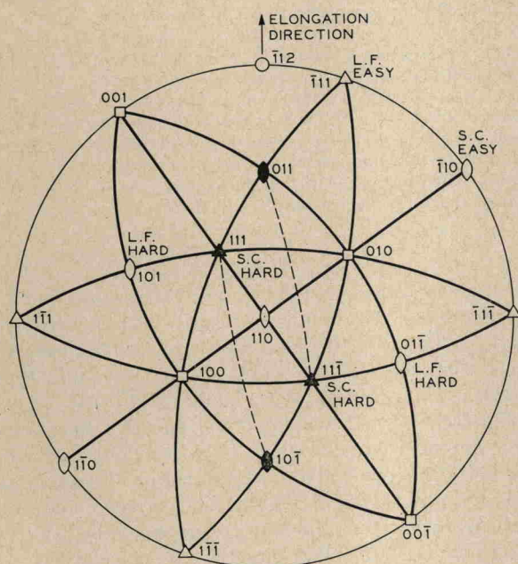
FIG. 1. (110) stereographic projection of a cubic crystal. During (110) [\bar{1}12] plane-strain compression, (111)[101] and (111)[011] slip systems become active. In L.F. deformation, [011] and [101] , which are perpendicular to the slip directions [011] and [101] , respectively, become hard axes, resulting in [\bar{1}11] being the easy axis. In S.C. deformation, the slip plane normals [111] and [\bar{1}1\bar{1}] are hard axes, leading to [\bar{1}10] as the easy axis.
